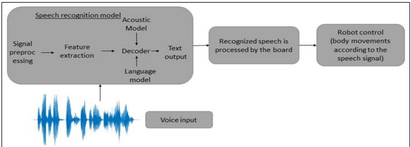
Fig 2 Block Diagram of Speech to Robot Body Movement Conversion
