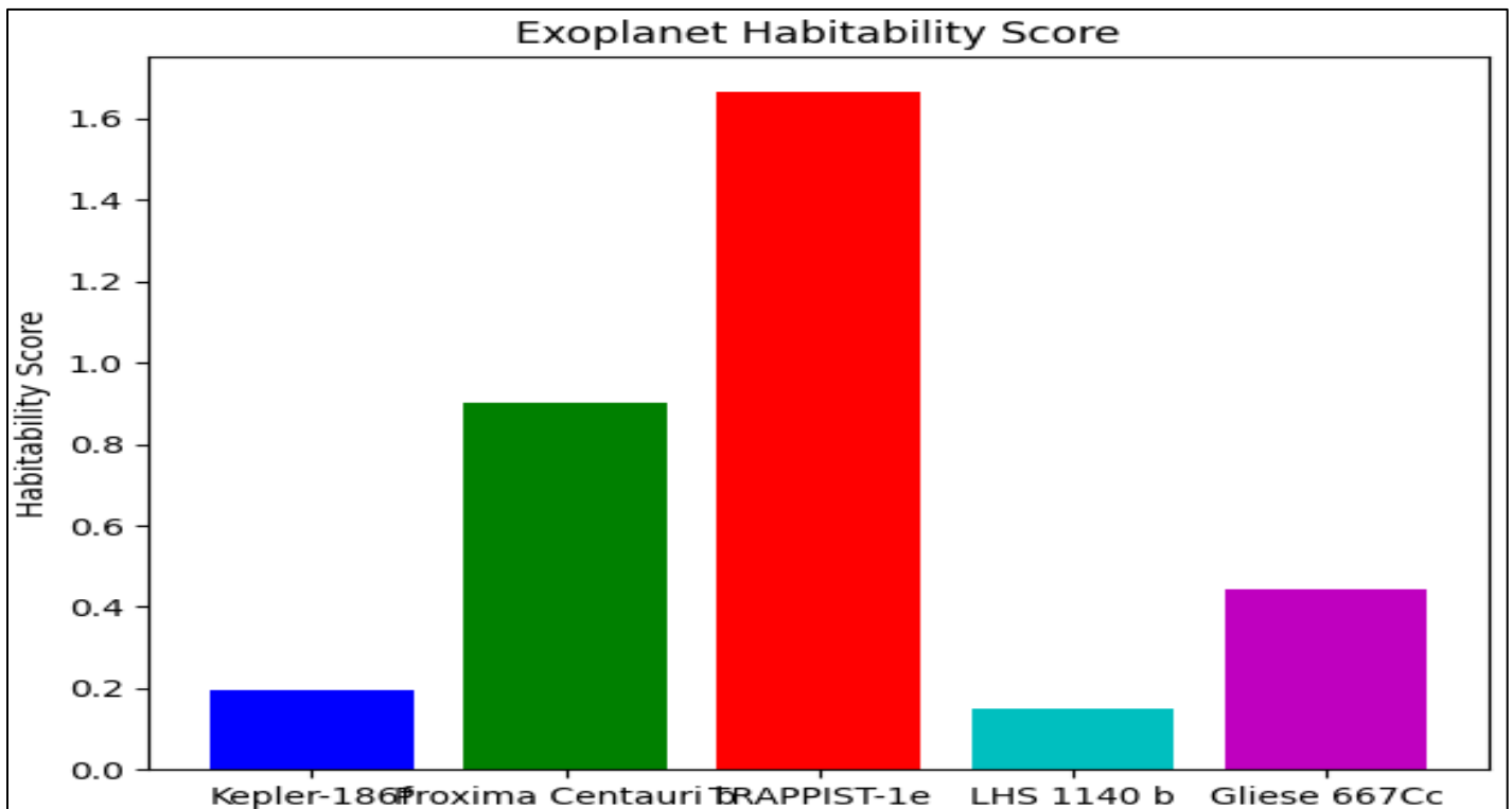
Fig 23: Habitability Score
