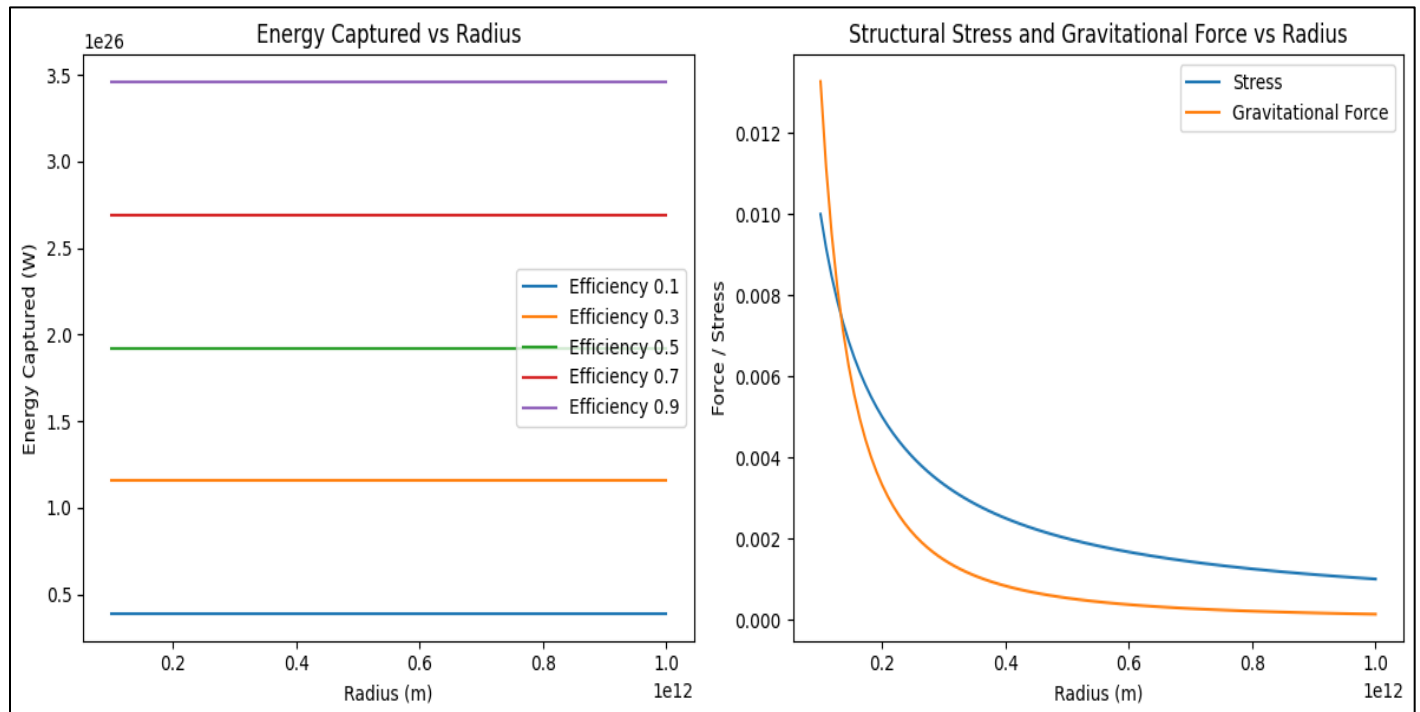
Fig 19: Energy Captured with various efficiencies, Structural Stress and Gravitational Plots based on the 4D Dyson Sphere's Radius)
