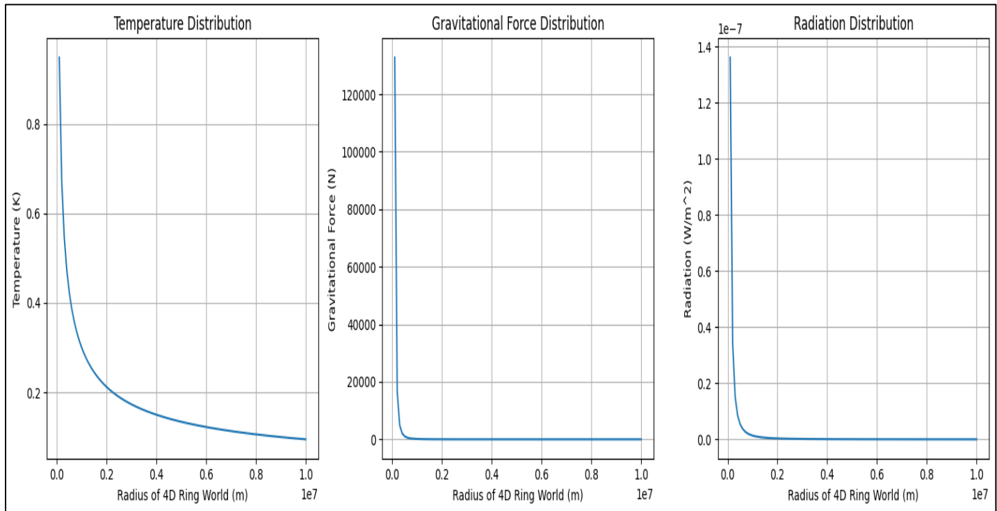
Fig 12: Implementing Radiation Distribution based on 4D ring worlds Temperature and Gravitational Distribution - Radiation: 0.00 \text{W/m}^2 )
