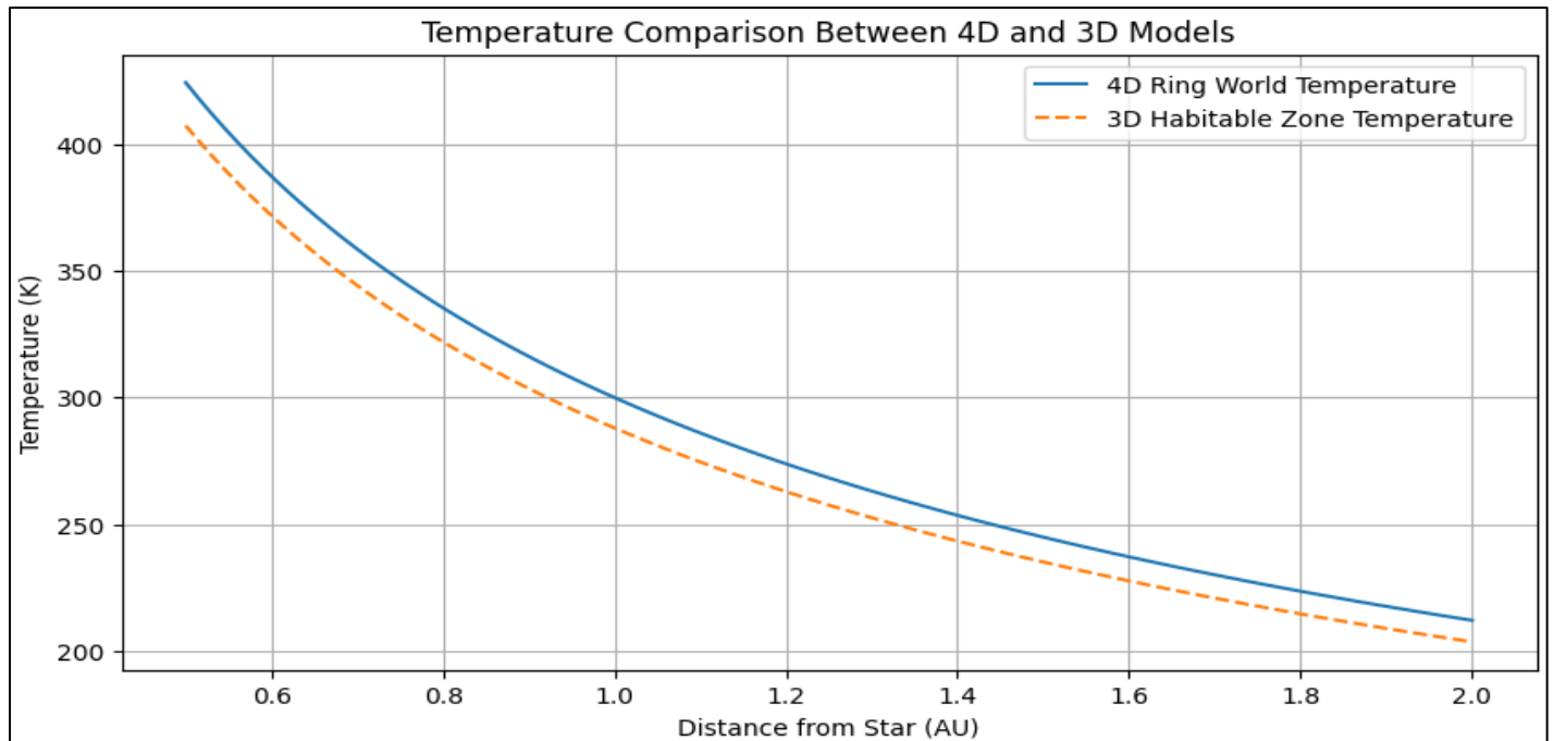
Fig 18: Habitable World Temperature Comparison between 3D and 4D Models Show Similar Trend But Small Difference in 4D Ring World Temperature that is Higher than that of 3D Habitable Zone Temperatures
