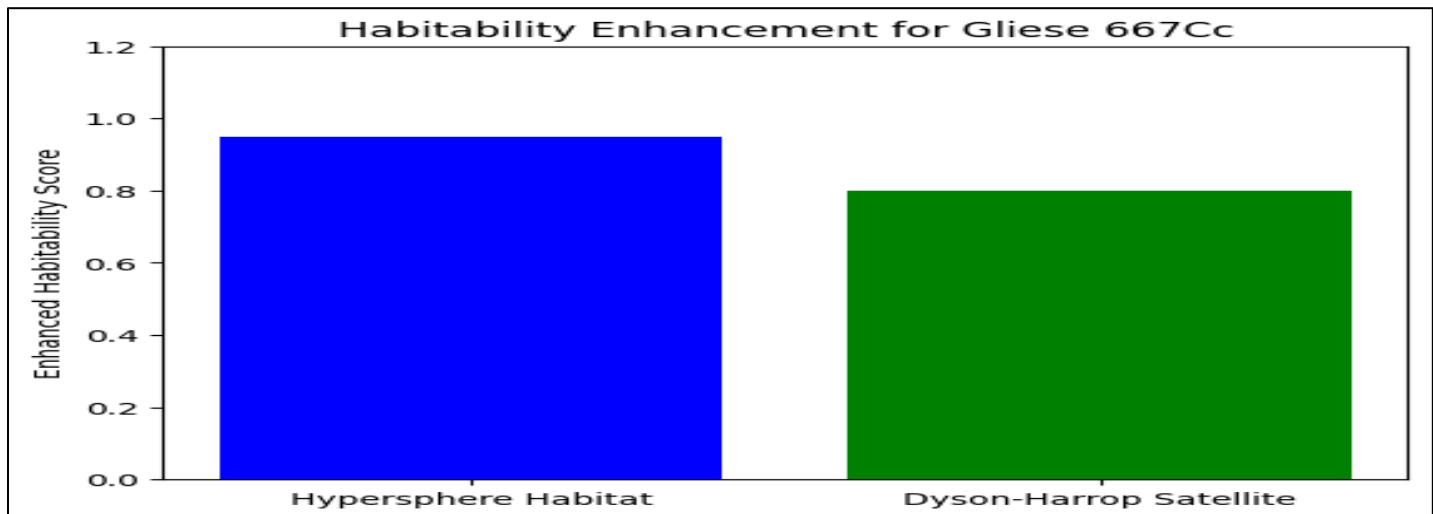
Fig 25: Hypersphere Habitat: Enhanced Habitability Score = 0.95 Dyson-Harrop Satellite: Enhanced Habitability Score = 0.80)
