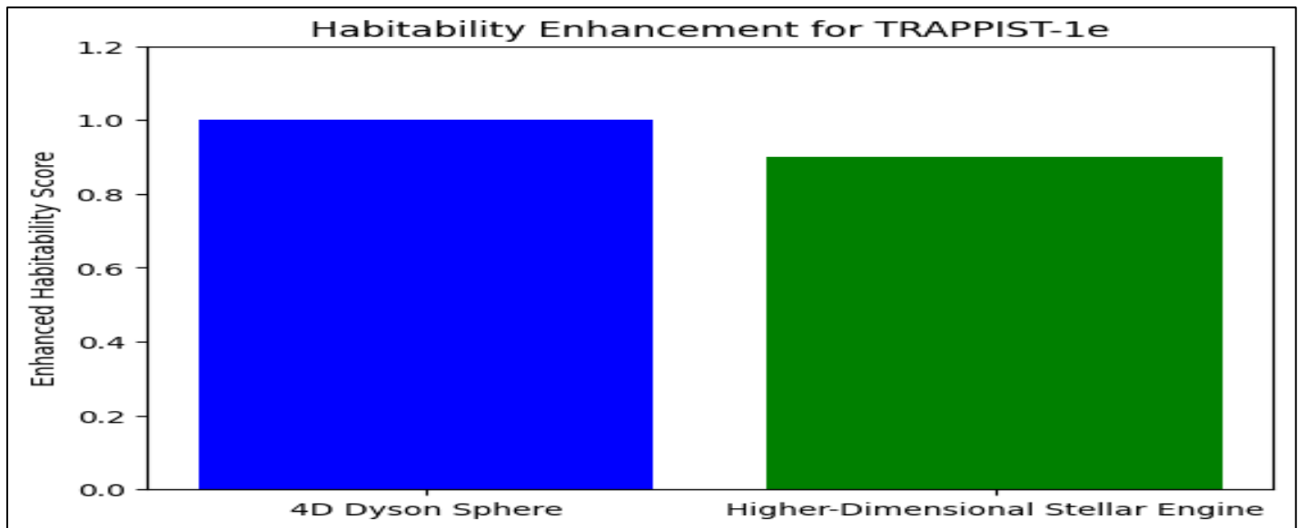
Fig 24: 4D Dyson Sphere: Enhanced Habitability Score = 1.00 Higher-Dimensional Stellar Engine: Enhanced Habitability Score = 0.90)
