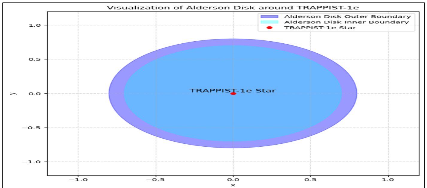
Fig 30: Visualization of Alderson Disk around Trappist- 1e
