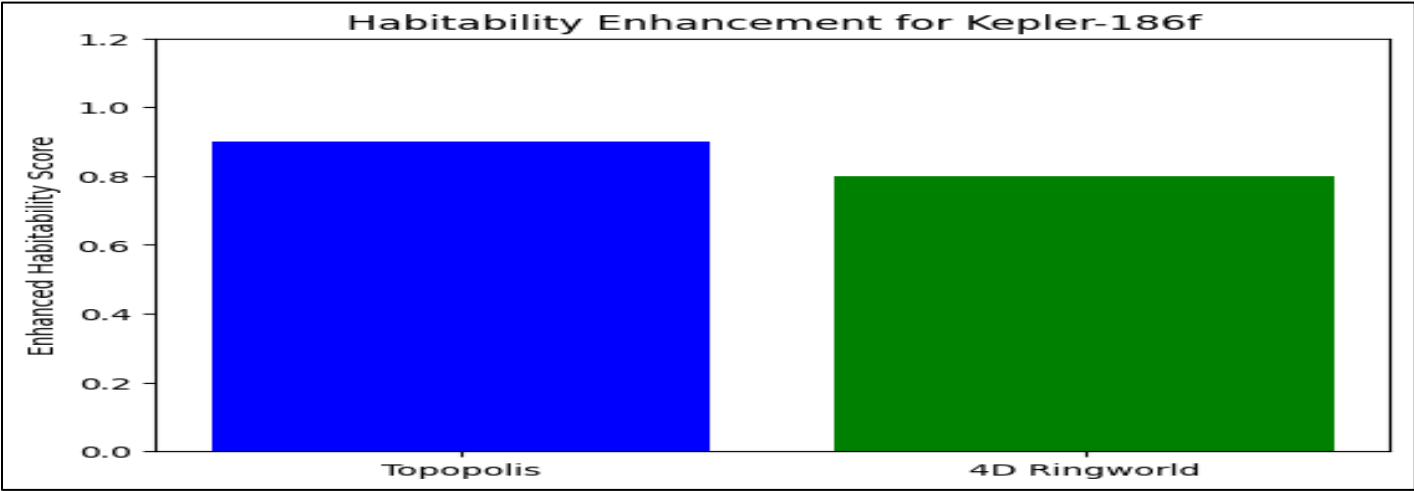
Fig 27: Topopolis: Enhanced Habitability Score = 0.90 4D Ringworld: Enhanced Habitability Score = 0.80)
