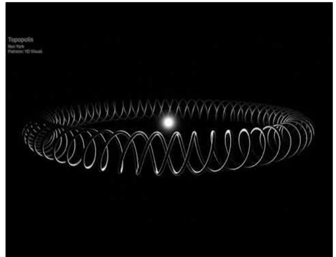
Fig 5: Speculated Topopolis
