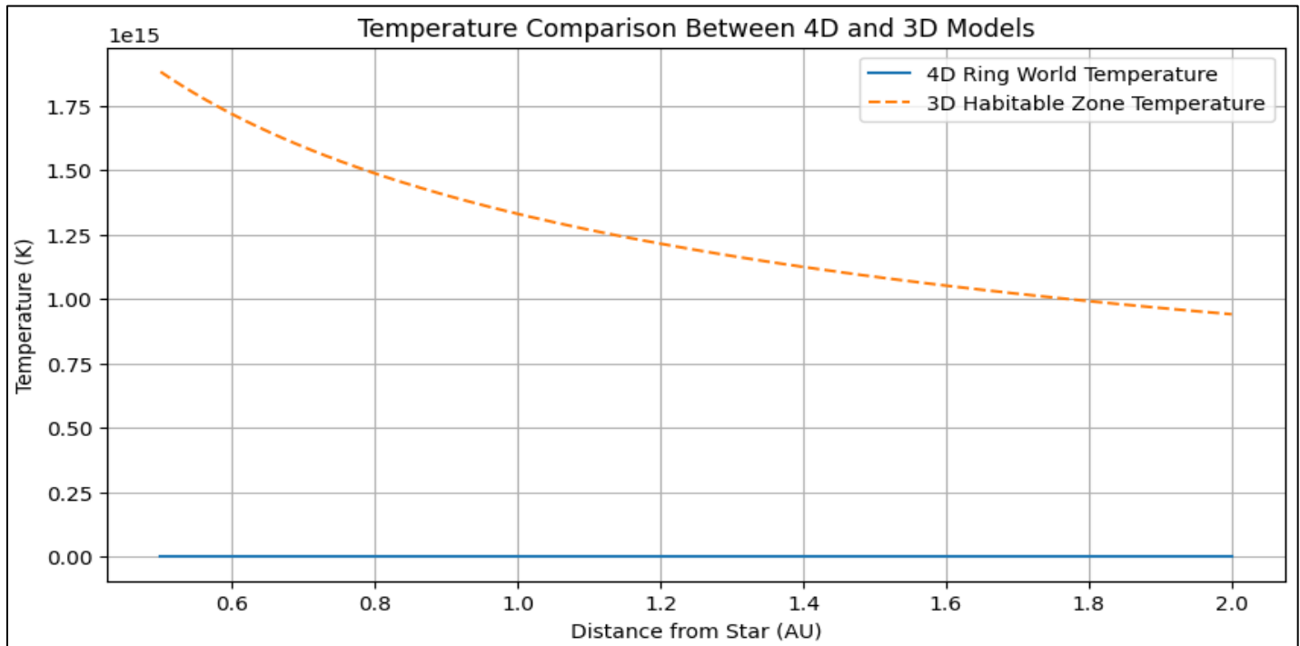
Fig 16: Temperature Comparison Plot
