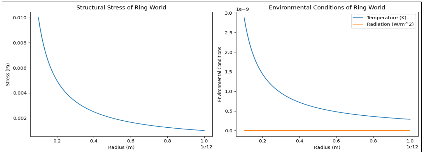
Fig 20: Structural Stress and Enviromental Conditions of 4D Ring World)
