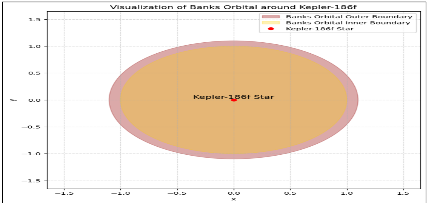
Fig 33: Visualization of Banks Orbital around Kepler 186f
