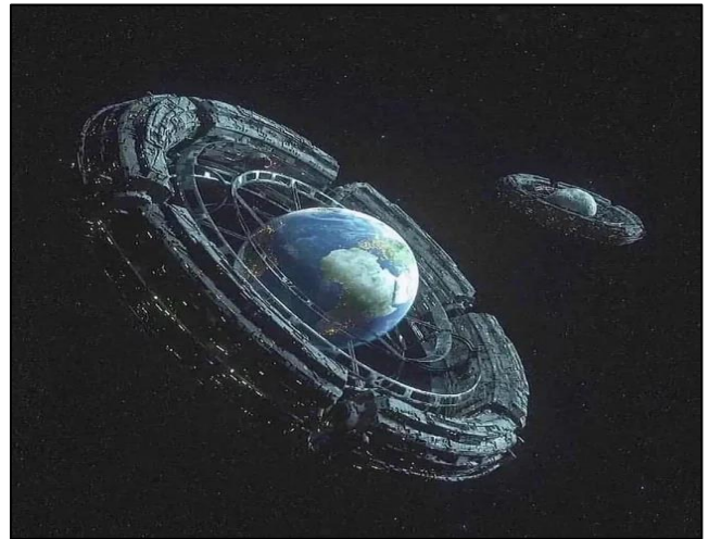
Fig 2: Possible Ring World Around Earth, if Conditions get Extreme for Human Life
