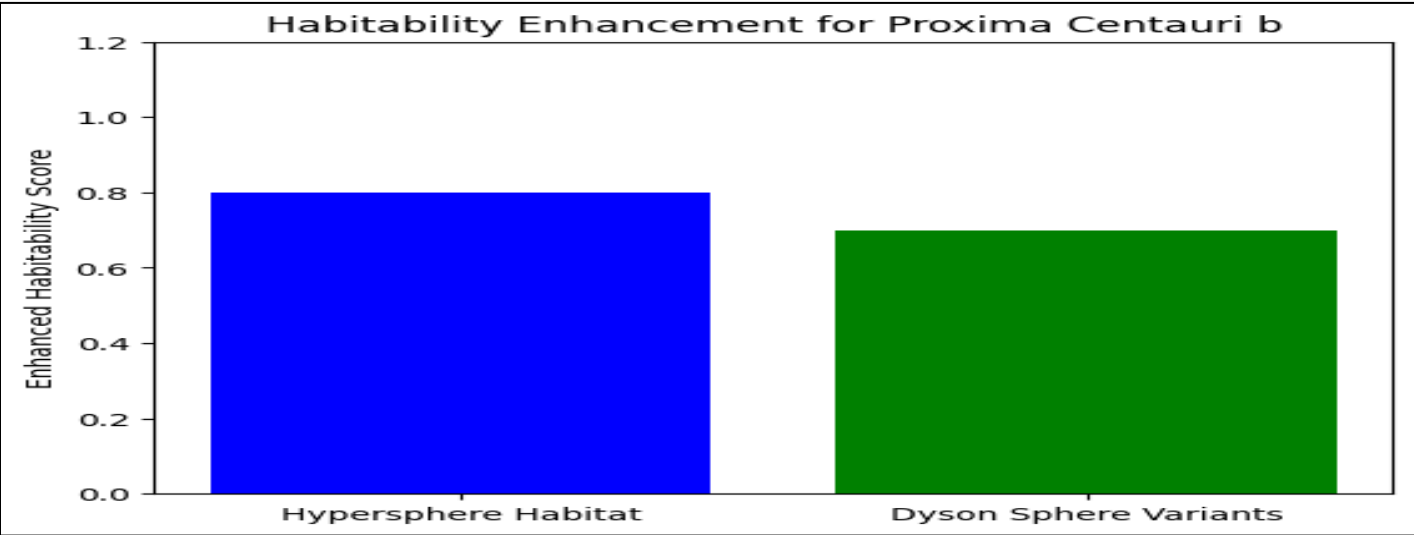
Fig 28: Hypersphere Habitat: Enhanced Habitability Score = 0.80 Dyson Sphere Variants: Enhanced Habitability Score = 0.70)
