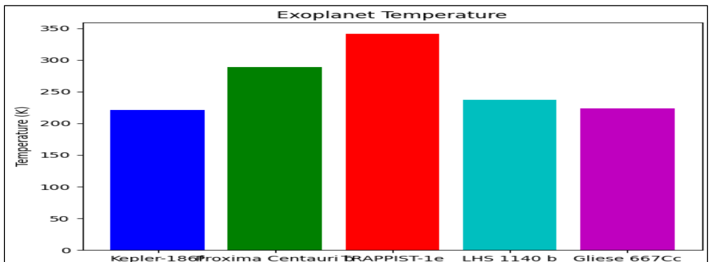
Fig 21: Based on Temperature
