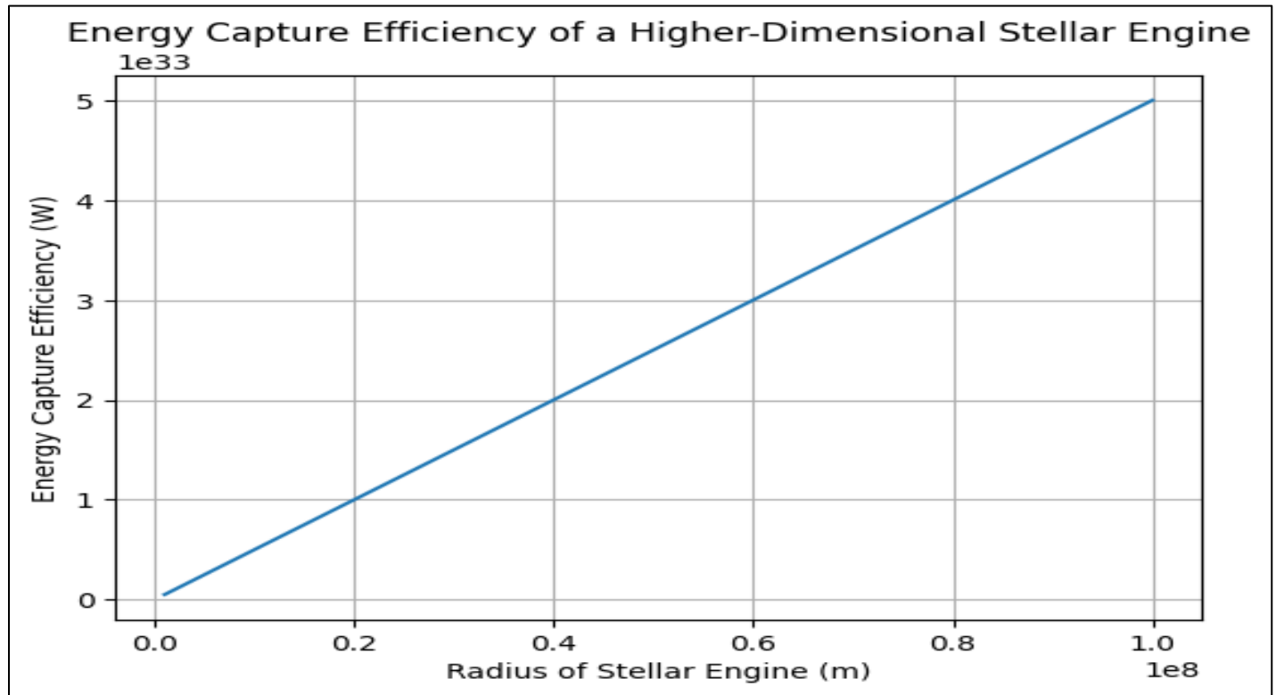
Fig 10: Energy Capture of Stellar Engine - 5.00 \times 10^{32} W)
