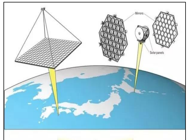
Fig 6: Dyson-Harrop Satellite
