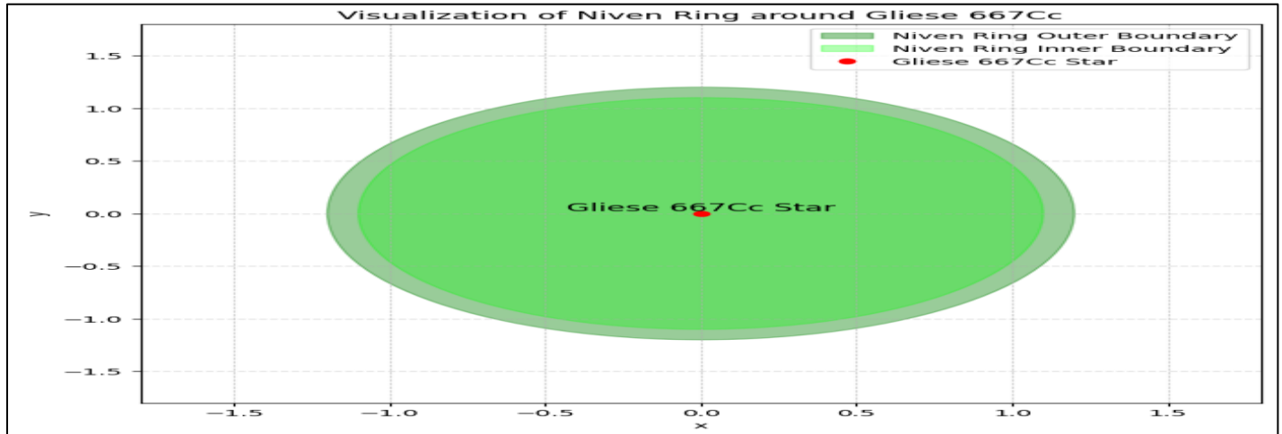
Fig 31: Visualization of Niven Ring around Gliese 667Cc
