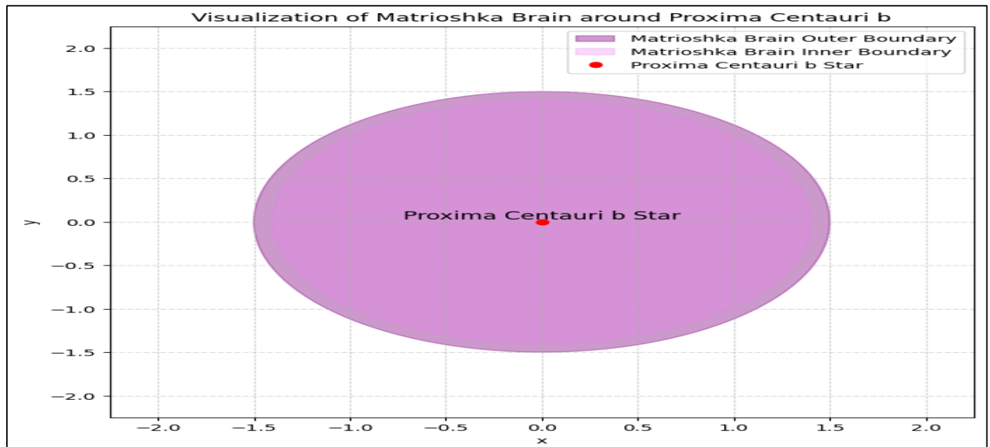
Fig 32: Visualization of Matrioshka Brain around Proxima Centauri b
