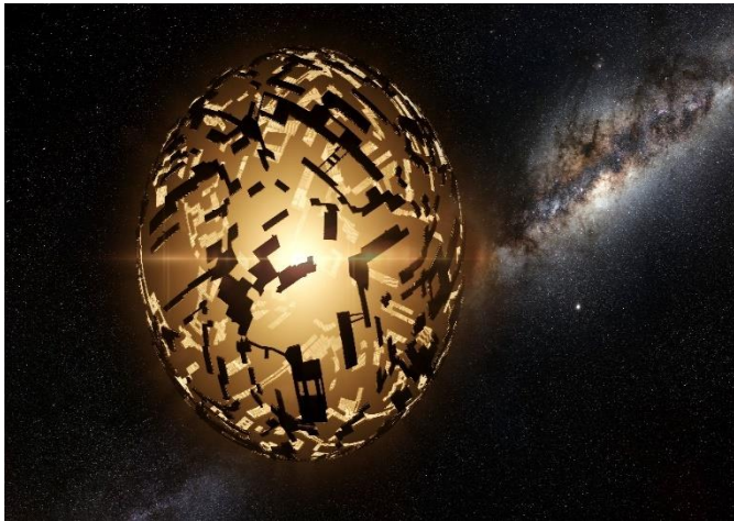
Fig 1: Possible Dyson Sphere Around Star
