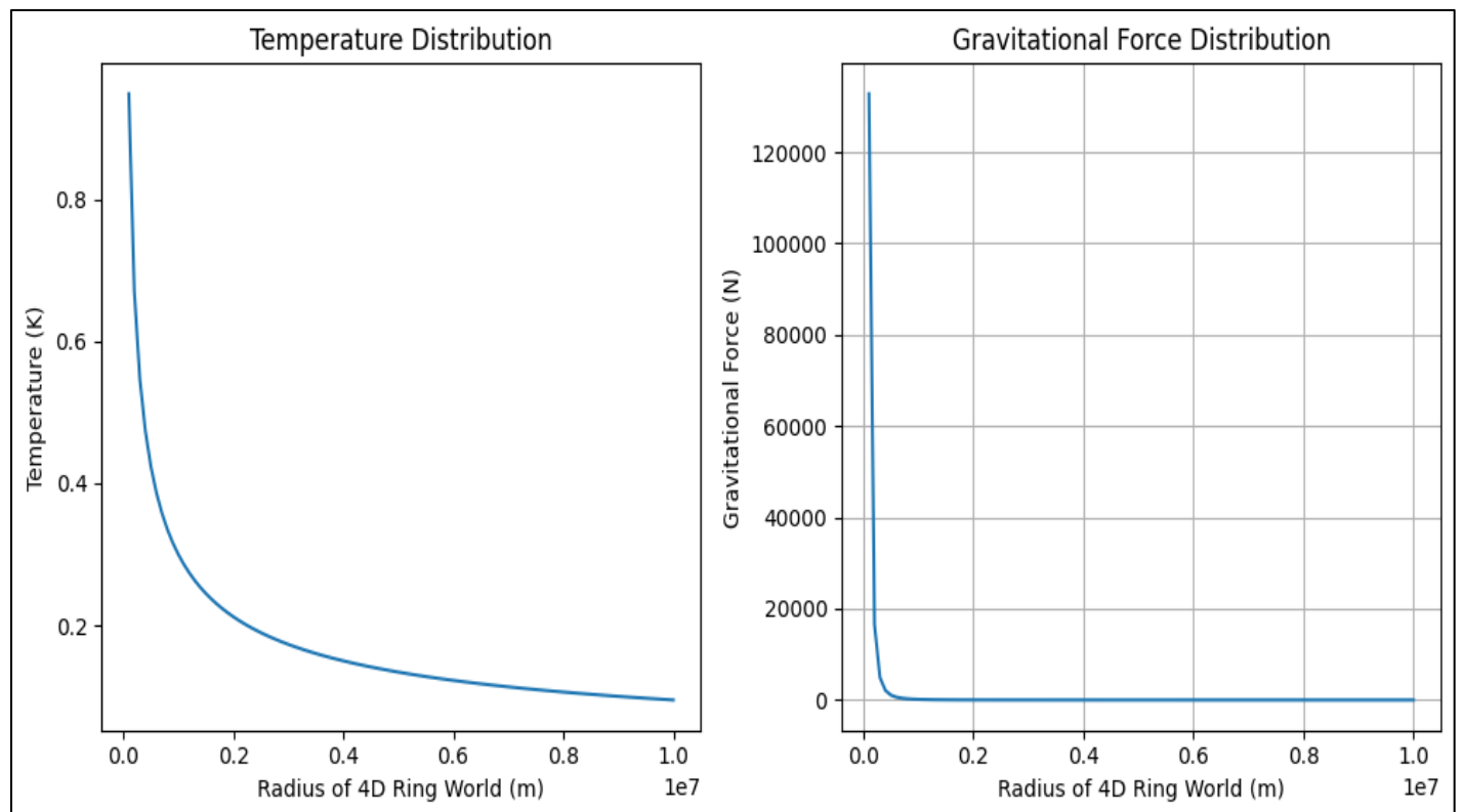
Fig 8: Temperature distribution of 4D Ring World - 0.30 K) Fig 9: Gravitational Force Distribution of 4D ring World - 1.33e+02 N
