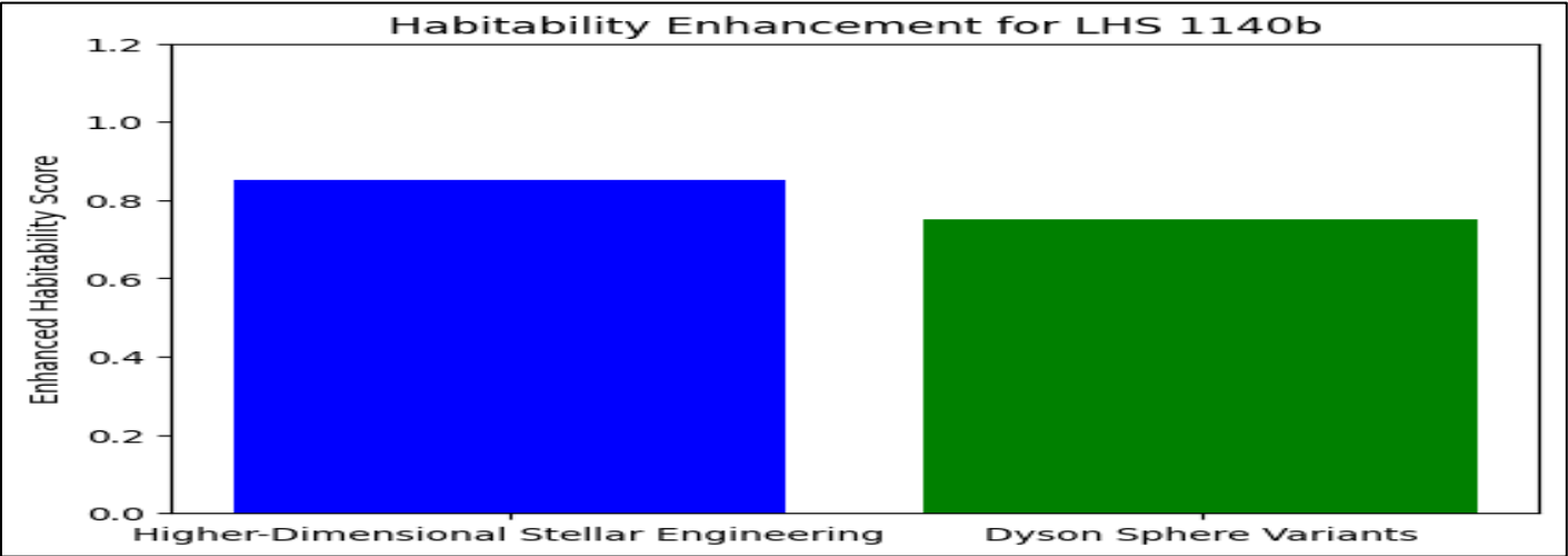
Fig 26: Higher-Dimensional Stellar Engineering: Enhanced Habitability Score = 0.85 Dyson Sphere Variants: Enhanced Habitability Score = 0.75)
