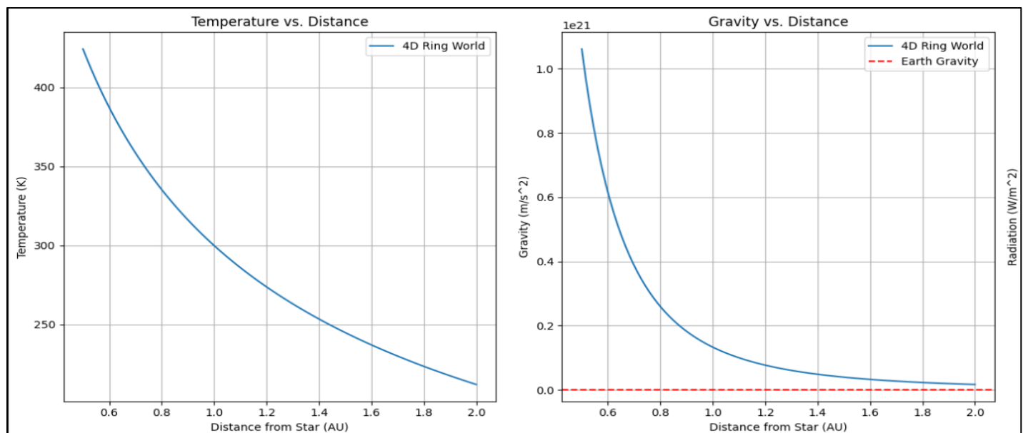
Fig 15: Comparing 4D Ring World Gravity to Earth's Gravity
