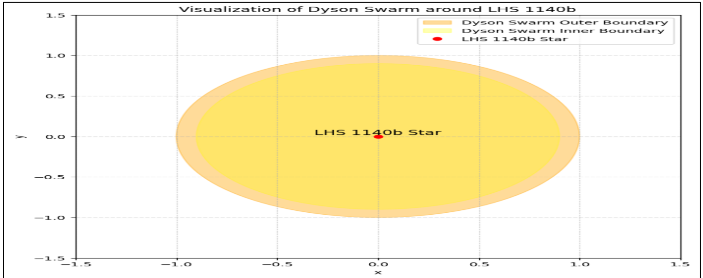
Fig 29: Visualization of Dyson Swarm around LHS 1140b
