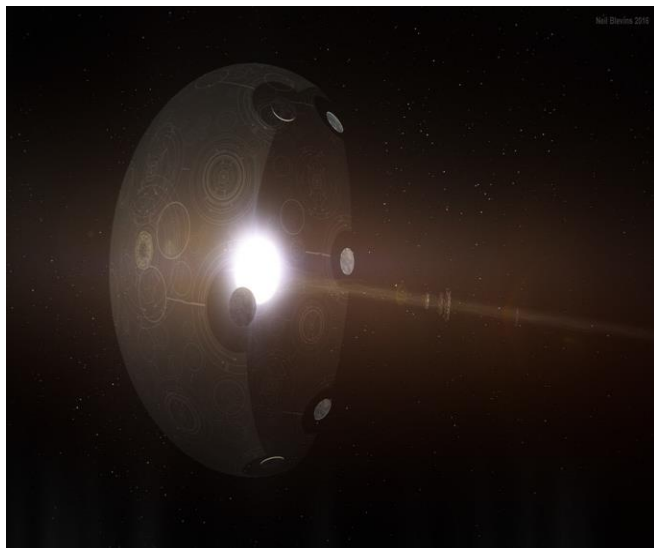
Fig 4: Speculative Shkadov Thruster
