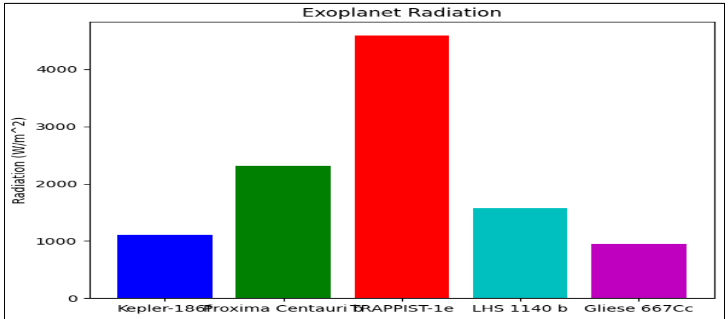
Fig 22: Based on Radiation
