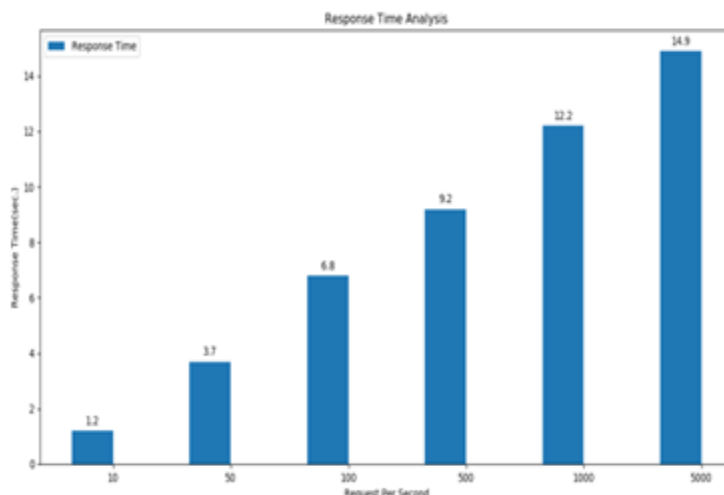
Fig 5 Response Time Analysis.
