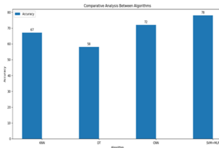
Fig 6 Comparative Analysis Between Algorithms
