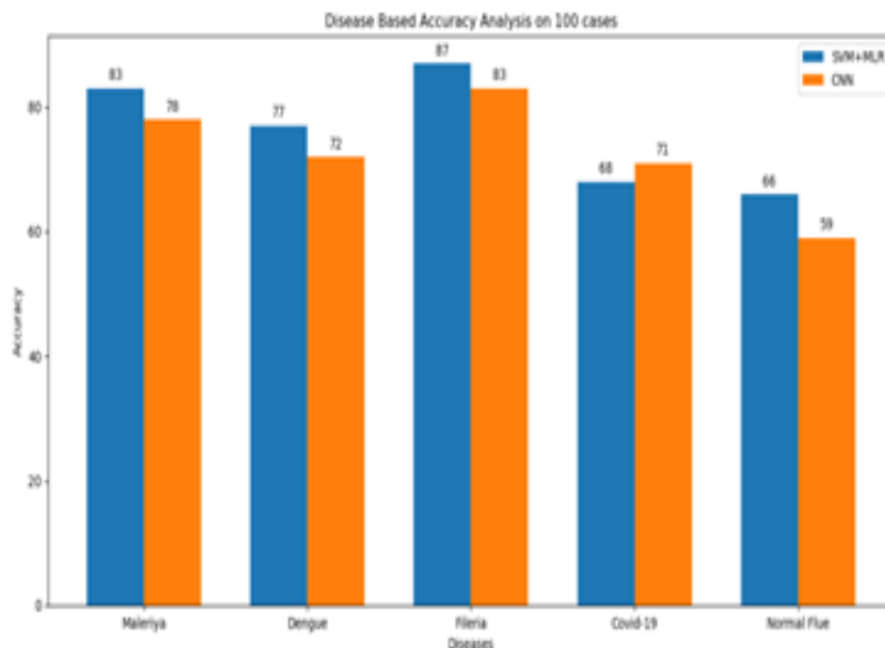
Fig 4 Disease Based Accuracy Analysis on 100 cases comparison.
