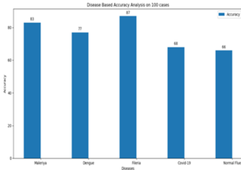
Fig 3 Disease Based Accuracy Analysis on 100 Cases Above Diagram Shows the Accuracy of 5 Diseases that are Malaria, Dengue, Filaria, Covid-19 and Normal Flu.
