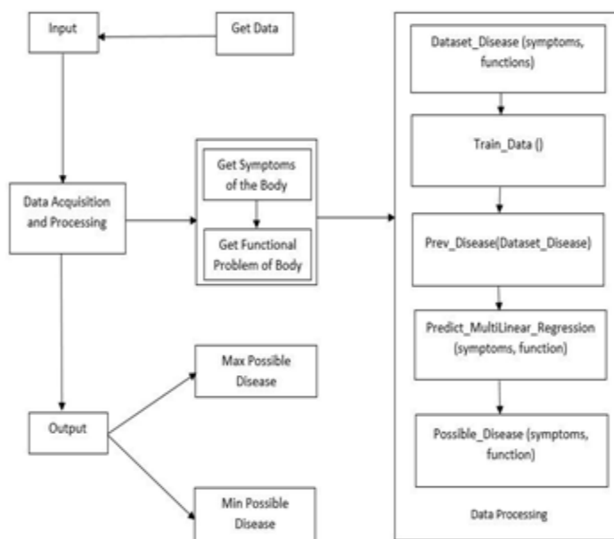
Fig 2 The Architecture of Disease Prediction System the Architecture of DPS Includes Multiple Following Fields.
