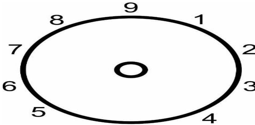
Fig. 1: (CSD)
