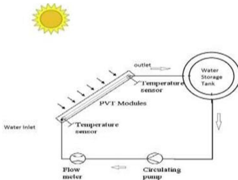
Fig 1 Schematic Diagram of the Experimental Test Setup
