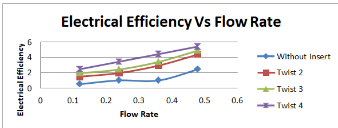
Fig 4 The Variation of the Electrical Efficiency with Flow Rate
