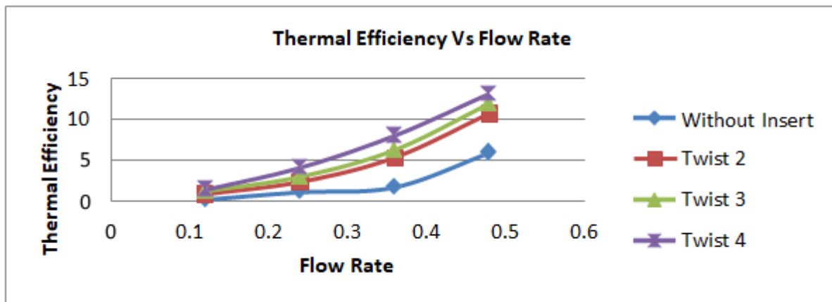
Fig 3 The Variation of the Thermal Efficiency with Flow Rate
