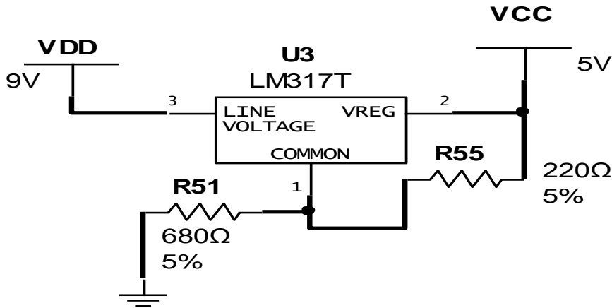
Fig 5 System 5V Power Supply
