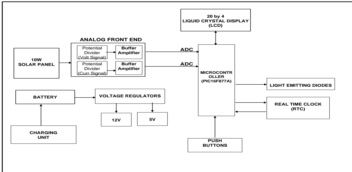
Fig 2 Basic Block Diagram of the System
