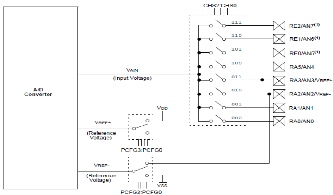
Fig 4 A/D Block Diagram of PIC16F876A
