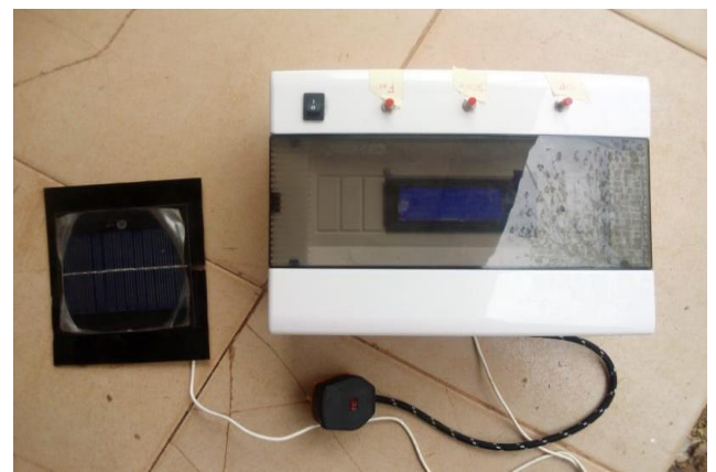
Fig 8 External View of the Developed Solar Data Logger
