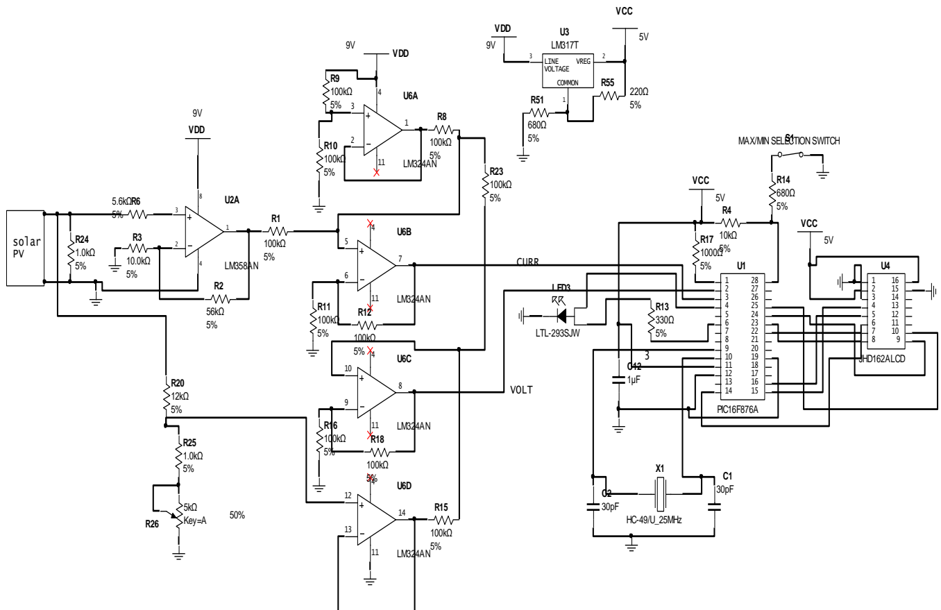
Fig 6 Complete Circuit Diagram of Solar Data Logger
