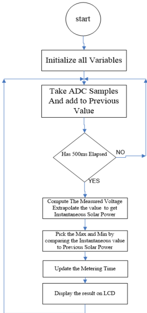
Fig 7 Flowchart of Solar Data Logger
