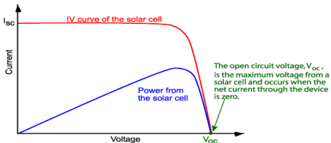
Fig 1 The Characteristic I-V Curve for Solar Cells (Honsberg et al.,2010)
