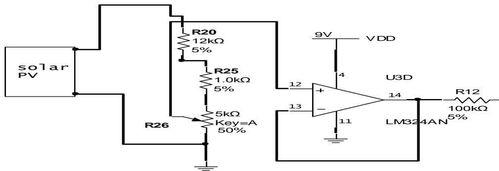
Fig 3 Voltage Sensing Circuit
