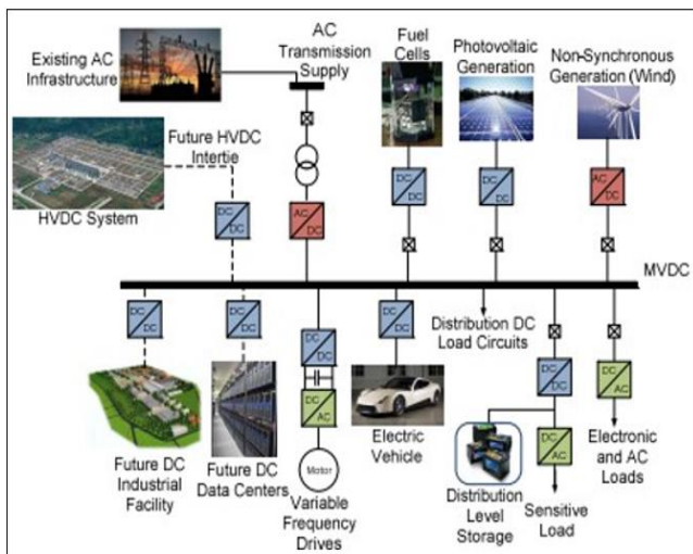
Fig 5 Implementation of Medium Voltage DC Grid for a Network of Stations
