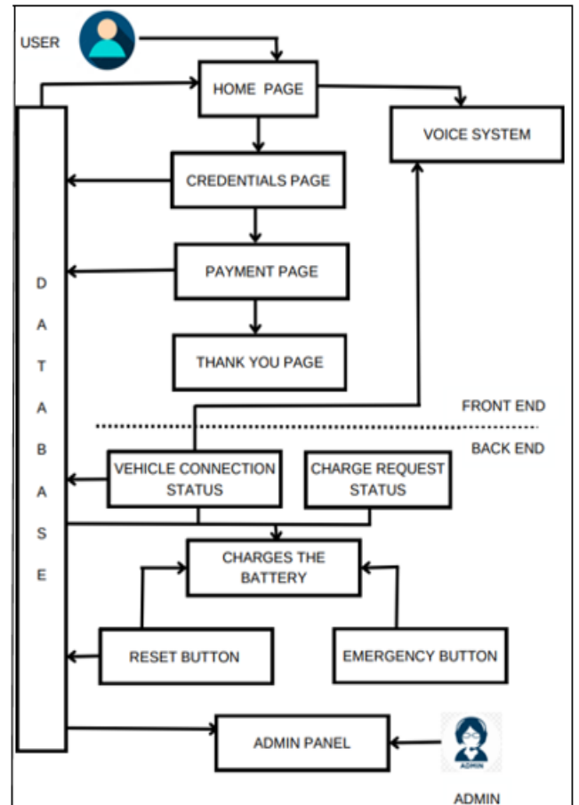
Fig 13 Software Dataflow for backend
