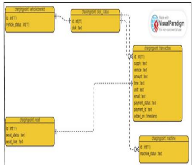
Fig 14 E-R diagram for our database
