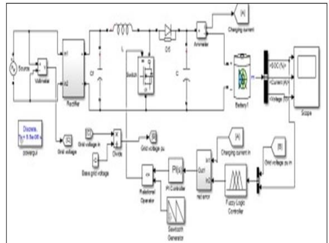
Fig 4 Simulation for Smart DC fast charging
