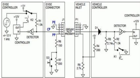
Fig 22 J1772 Standard EV Charging Connections
