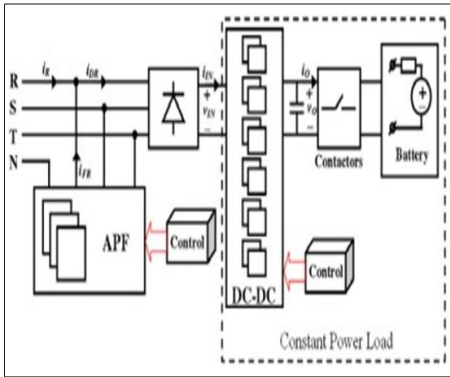
Fig 3 Block Diagram for DC fast charging implementation
