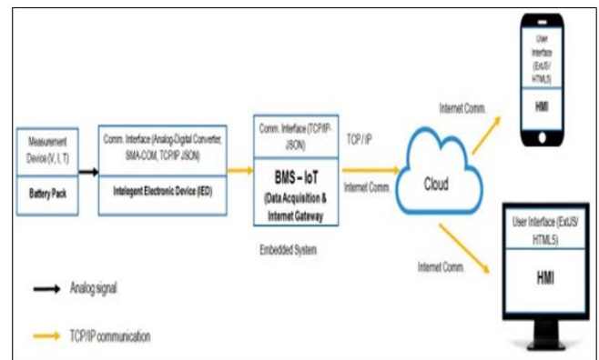
Fig 6 Proposed Blockdiagram of a IoT Battery pack
