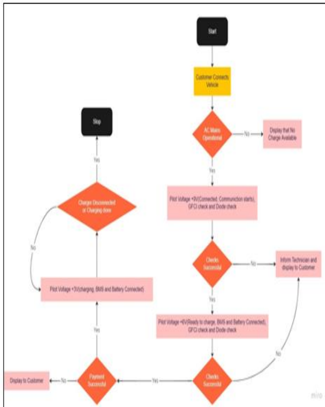
Fig 16 Pilot Algorithm
