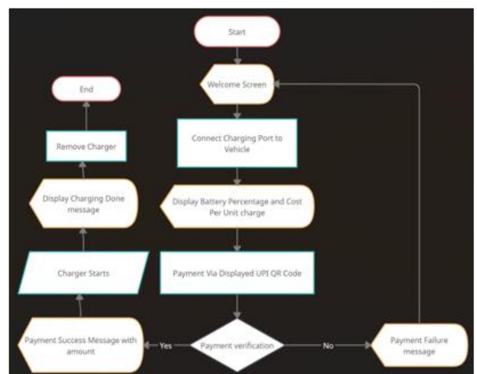
Fig 8 Client Side Flow
