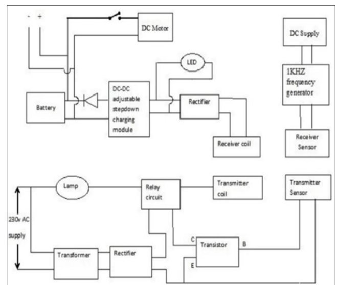
Fig 1 Proposed Block Diagram of Smart Charging For Electric Vehicles
