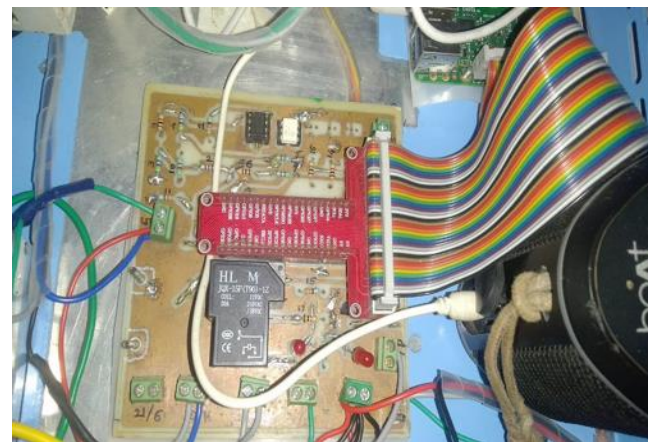
Fig 11 Pilot communication and Vehicle verification circuit
