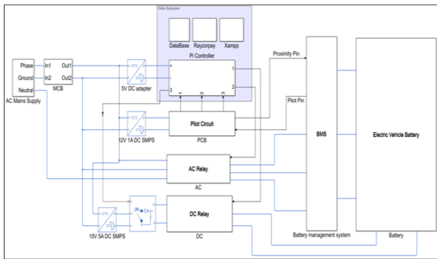
Fig 9 Functional Block Diagram of system
