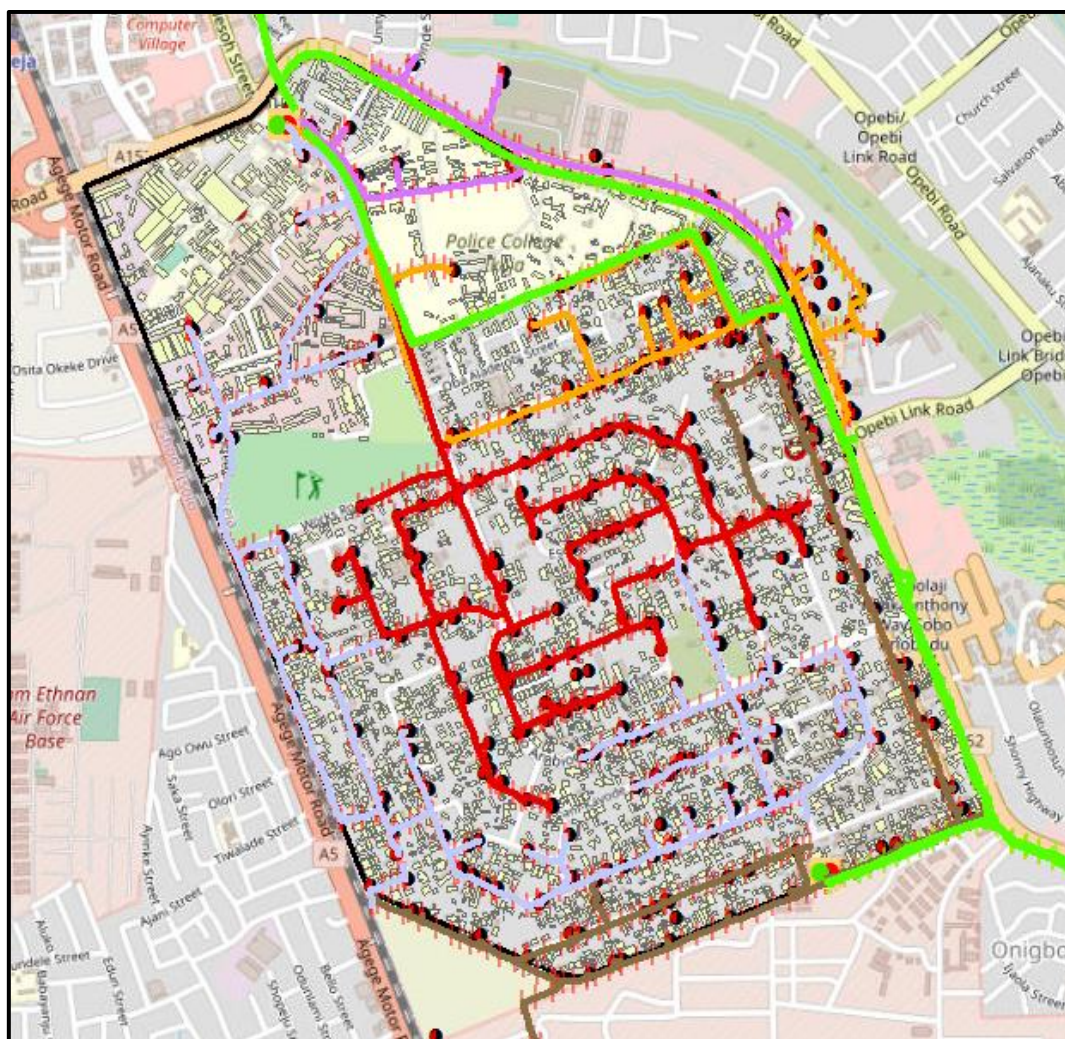
Fig. 17(a): 11kV Poles and Lines and 33/11kV Distribution Transformers
