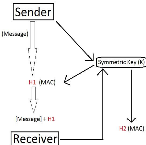
Fig 3. Implementation Diagram
