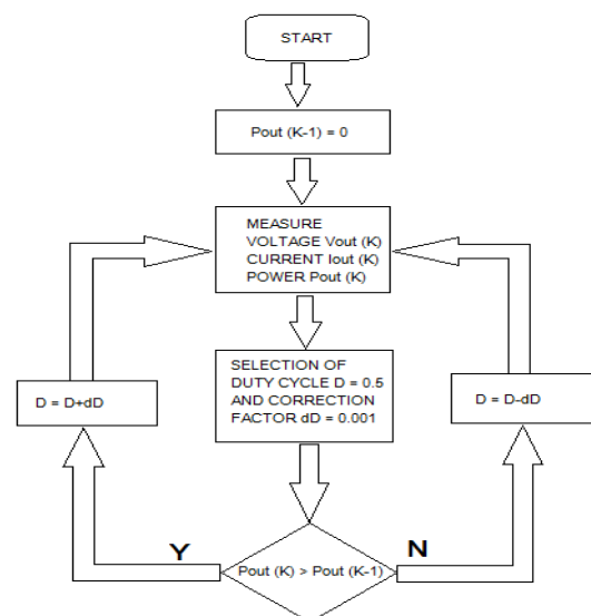
Fig 3:- Algorithm of implemented MPPT-1
