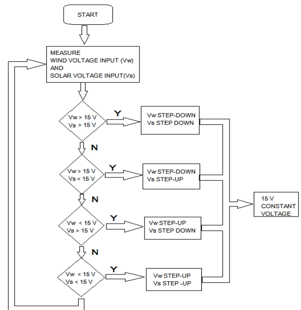
Fig 2:- Algorithm of implemented MPPT-1
