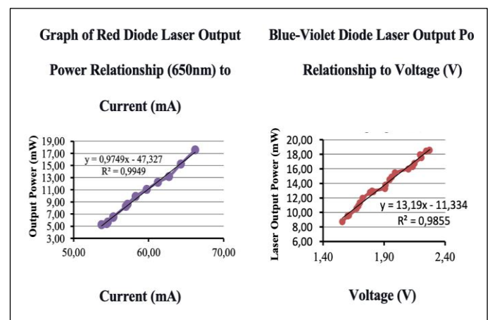
Fig 3. Graph of Relationship of 650nm Red Laser Power and Current (left) and Graph of Relationship of Blue-Violet Laser Power (405nm) with Voltage (right)
